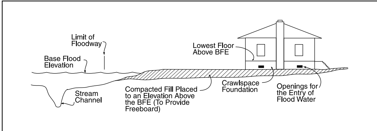
Figure 3 Structure on a crawspace foundation. The lowest floor is raised above the BFE. Openings in the foundation walls allow water from floods higher than the fill elevation to enter the crawspace and equalize the pressure on foundation walls.
